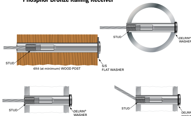
Phosphor Bronze Railing Receiver
